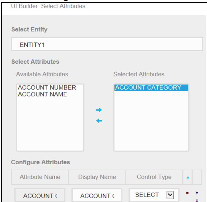
Figure 5: Select Attributes
